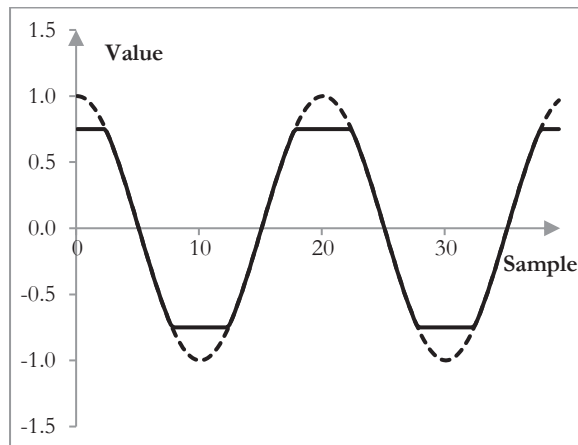
Figure 18. Hard clip of a simple wave
